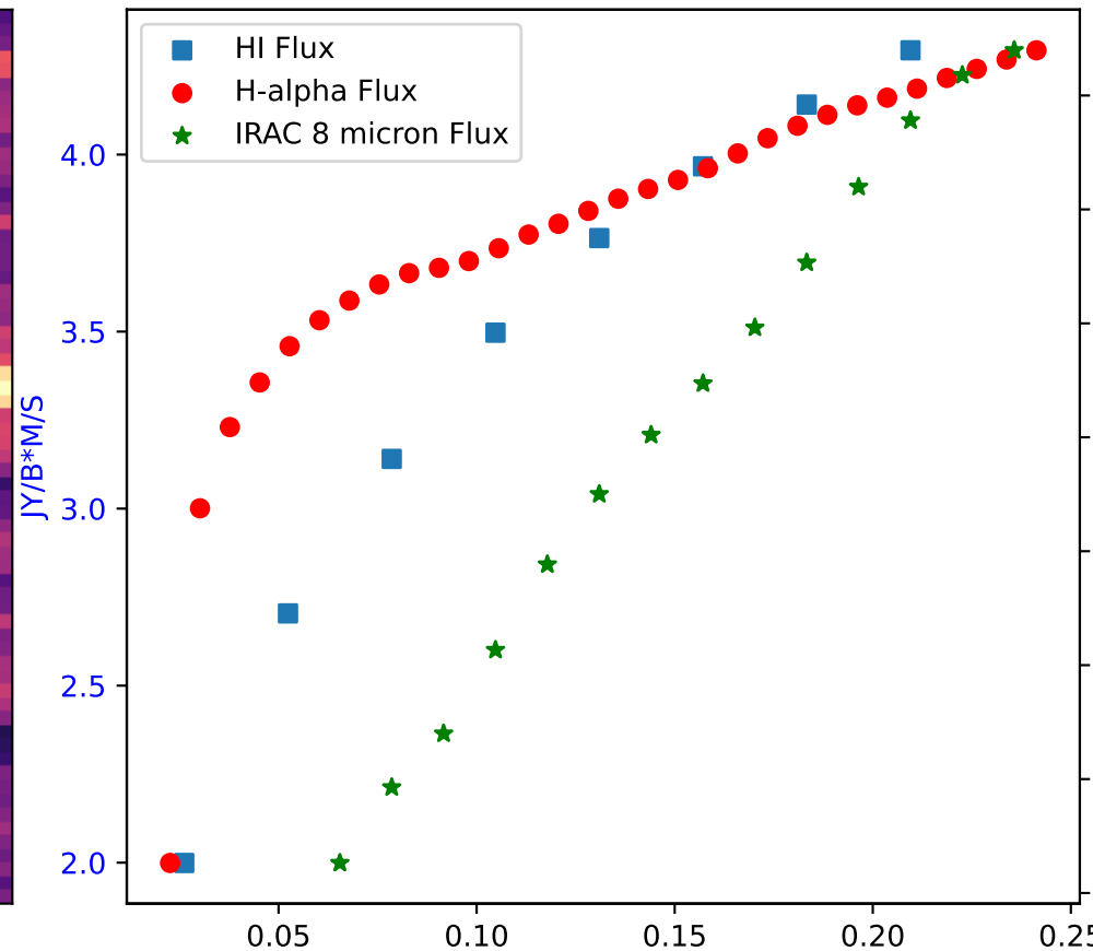
Flux of HI vs. H-alpha in Galaxy: DDO 53 - Region 6
